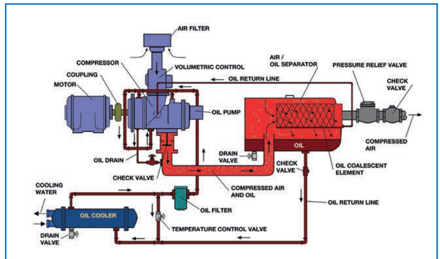
Flow diagram for oil-flooded rotary screw air compressor
